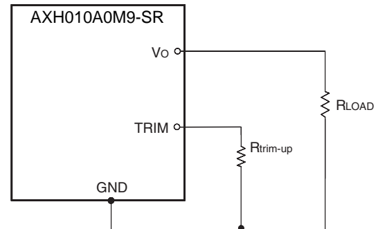
Figure 21. Circuit Configuration to trim-up output voltage.
