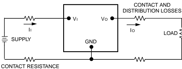
Figure 16. Peak-to-Peak Output Ripple Measurement Test Setup.
