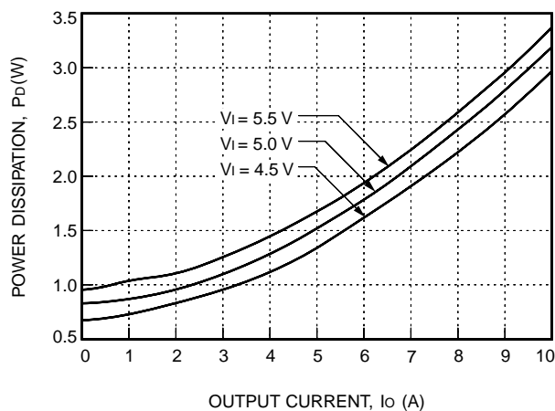
Figure 46. NH033G-L Typical Power Dissipation vs. Output Current, T_A = 25^\circ\text{C}
