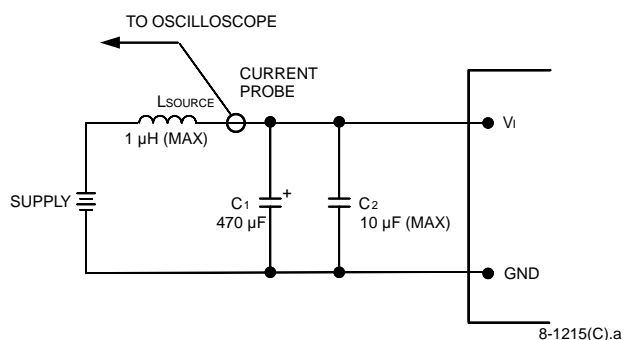
Figure 36. Setup with External Capacitor to Reduce Input Ripple Voltage
