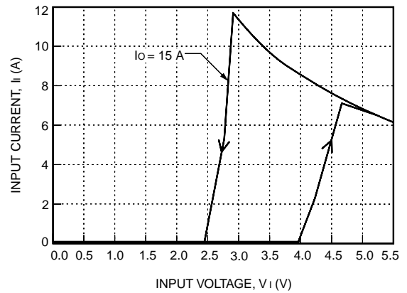
Figure 4. NH050S1R8-L Input Characteristics, T_A = 25\text{ }^{\circ}\text{C}
