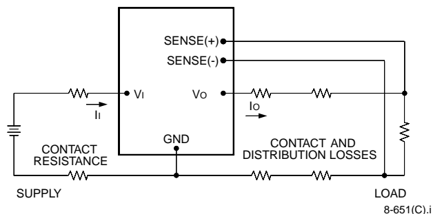
Figure 39. Effective Circuit Configuration for Single-Module Remote-Sense Operation
