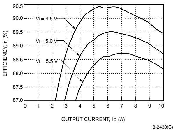
Figure 21. NH033G-L Efficiency, T_A = 25^\circ\text{C}
