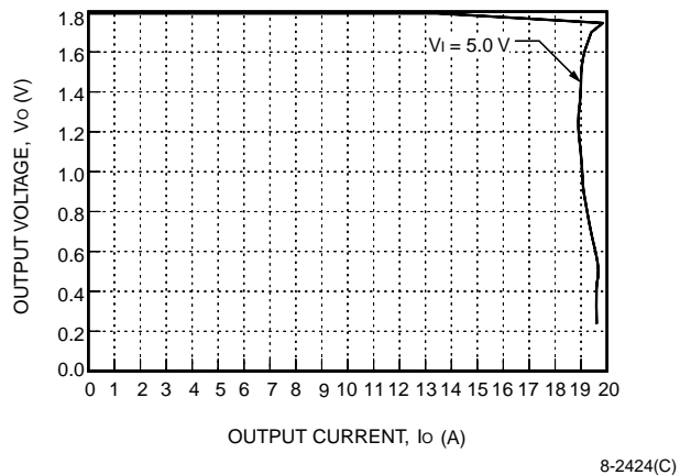
Figure 11. NH033S1R8-L Current Limit, T_A = 25\text{ }^{\circ}\text{C}
