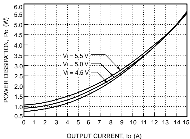
Figure 45. NH050S1R8-L Typical Power Dissipation vs. Output Current, T_A = 25^\circ\text{C}
