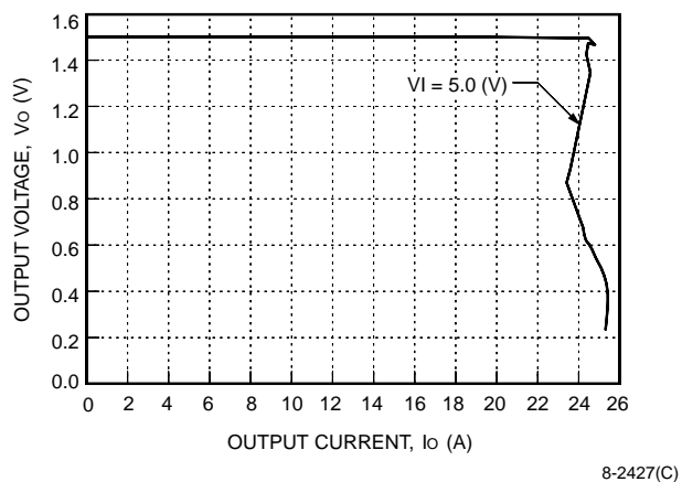
Figure 10. NH050M-L Current Limit, T_A = 25\text{ }^{\circ}\text{C}
