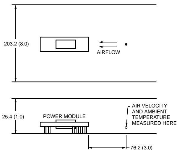
Figure 40. Thermal Test Setup
